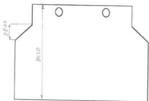
Cargo Hold 2 (Mid) Sectional view
