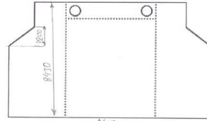
Cargo Hold 1 (Fore) Sectional view
